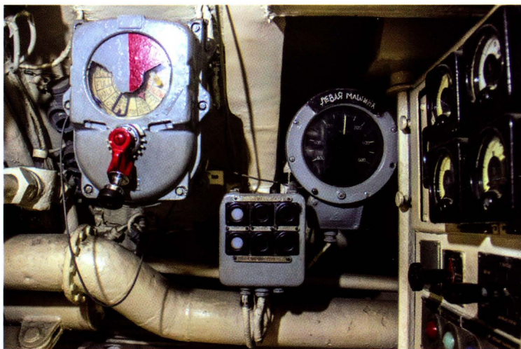
Alat Pengukur Kecepatan dan Arah Kapal Equipment to Measure Boat Speed and Orientation
